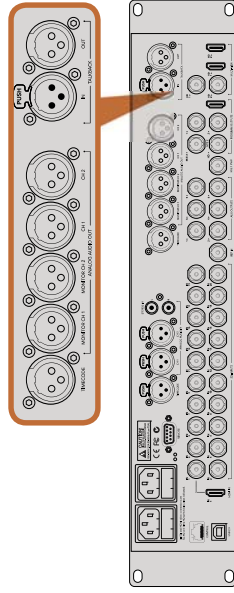
ATEM 2 M/E Production Studio 4K features built in XLR connectors for timecode, audio and talkback
